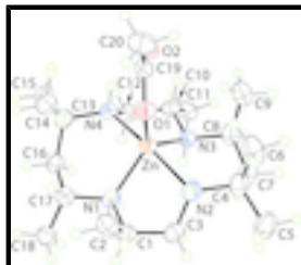
Fig. 1. The molecular structure of (I) showing the atom-labelling scheme and displacement ellipsoids at the 50% probability level. The perchlorate counter-ion is omitted.
