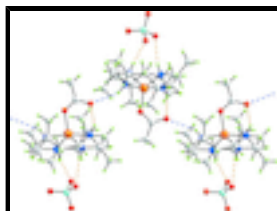
Fig. 2. Helical supramolecular chains in (I) sustained by N-H\cdots O(\text{acetate}) hydrogen bonds (blue dashed lines). Associated with these chains are the perchlorate anions held in place by N-H\cdots O interactions (orange dashed lines).
